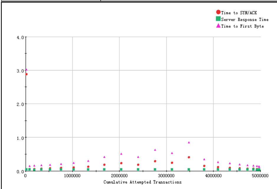
Real Time Statistics - Network Response Time vs. Load
