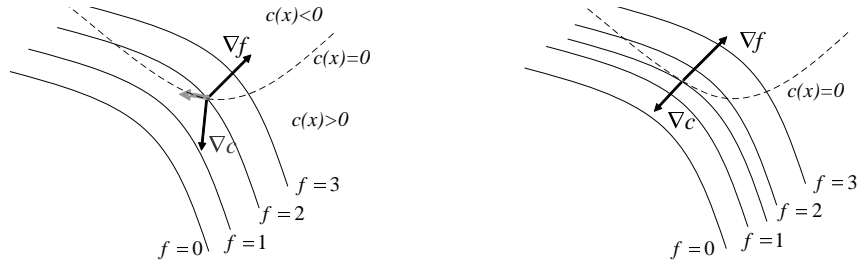
Fig. 1. At the constrained optimum, the gradient of the constraint must be parallel to that of the function.
